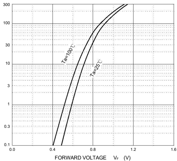
Forward Characteristics
