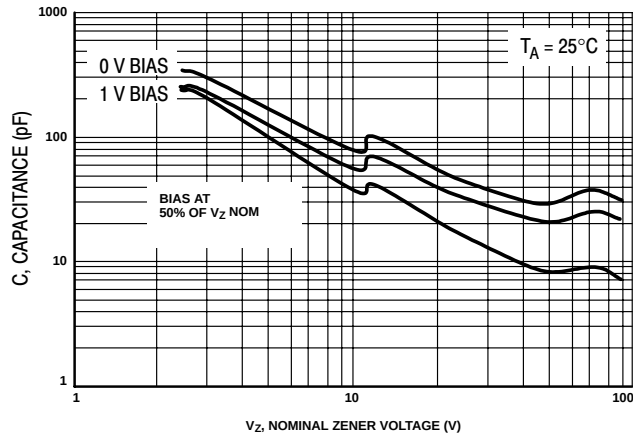
Figure 5. Typical Capacitance
