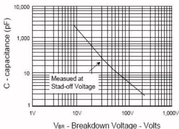
Fig. 3 - Typical Capacitance vs. Breakdown Voltage
