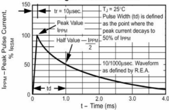
Fig. 3 – Pulse Waveform
